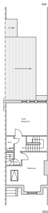
Existing Second Floor Plan
